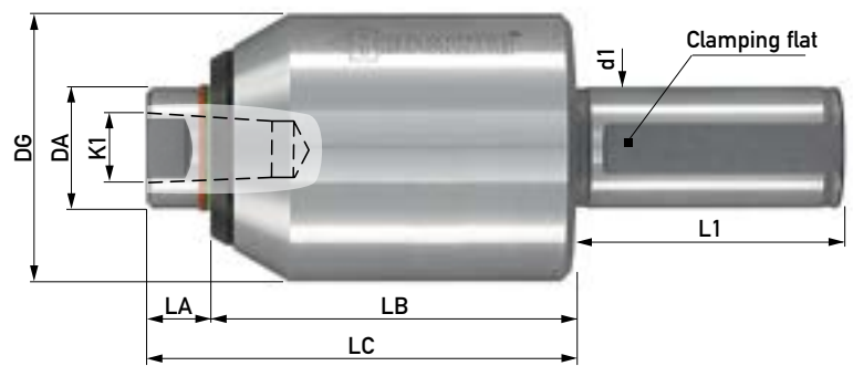
Interchangeable inserts for type TRE on page 35
