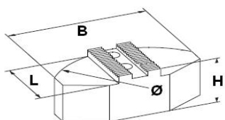
Segmentbacken, Ø 3 Backen = 380mm / Pie Jaws Ø 3 Jaws = 380mm
