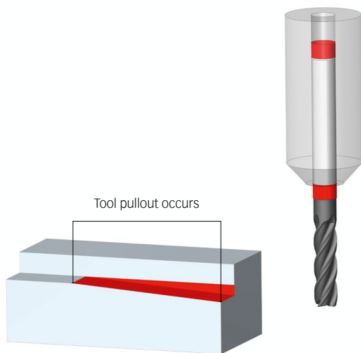
Length alterations can lead to damage of the workpiece.
