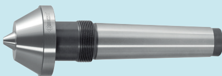
double diameter 60° dead centre with draw-off thread
