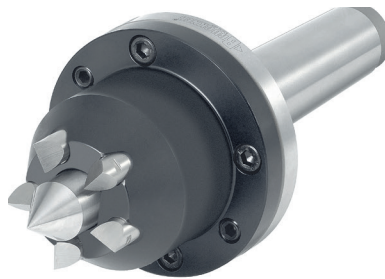
SM Face Drivers with mechanical compensation
