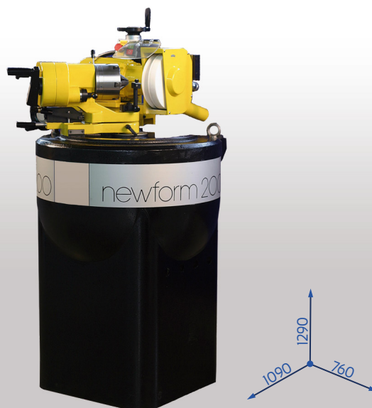
Dimensioni senza Lampada LED / Dimensions without LED Lamp
