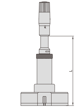
Type C 50-200mm, carbide measuring points three points
