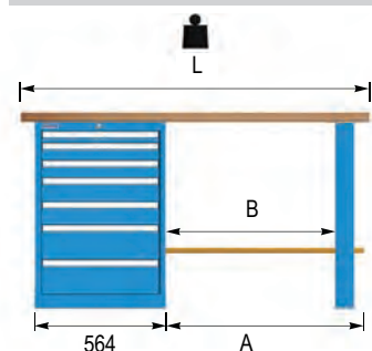
1 Leg and 1 Drawer cabinet 27x36 Eh
