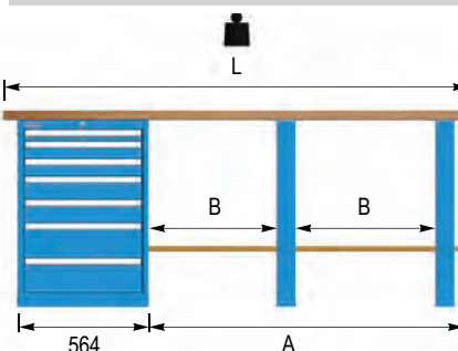
2 Legs and 1 Drawer cabinet 27x36 Eh
